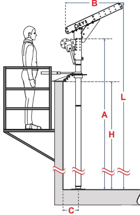
800 kg kapasiteli manuel el vinci Hand winch with 800 kg capacity
